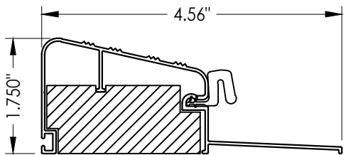
78 OUTSWING THRESHOLD
