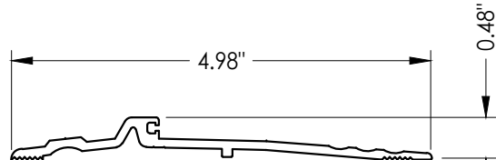
40 THRESHOLD
