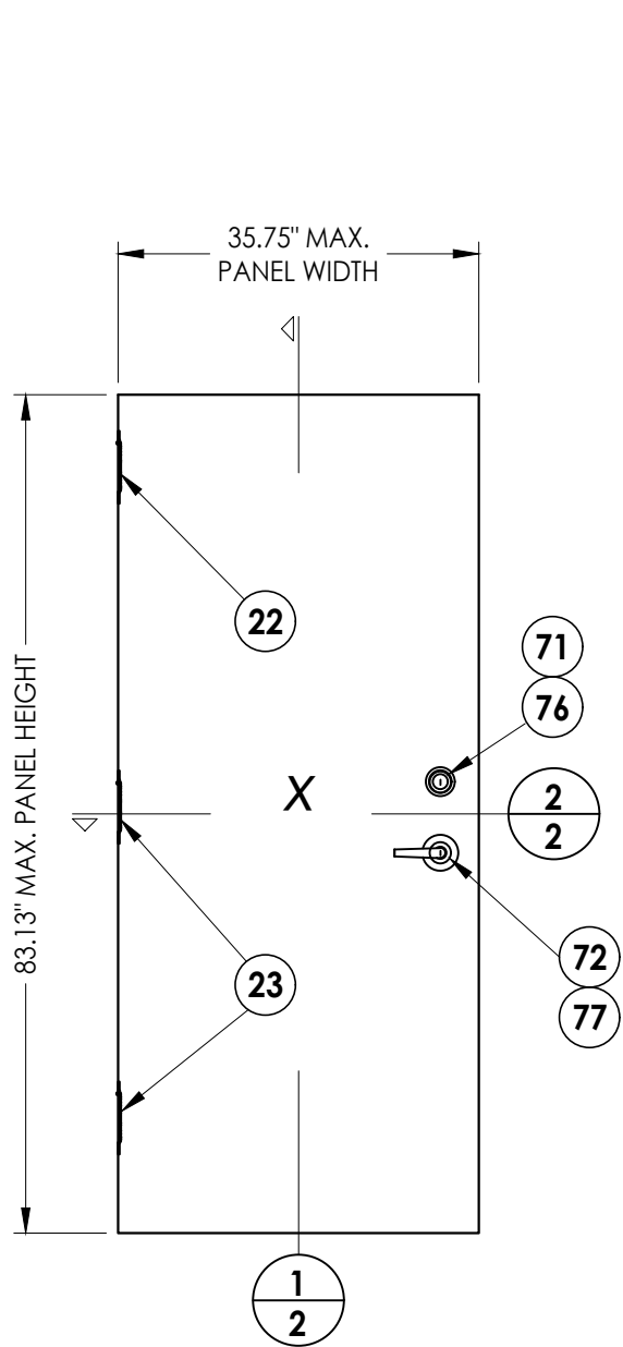
1 "N" OPAQUE STEEL DOOR PANEL
