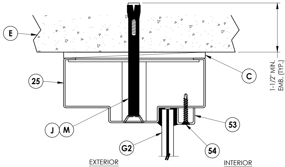
1 5 VERTICAL CROSS SECTION
